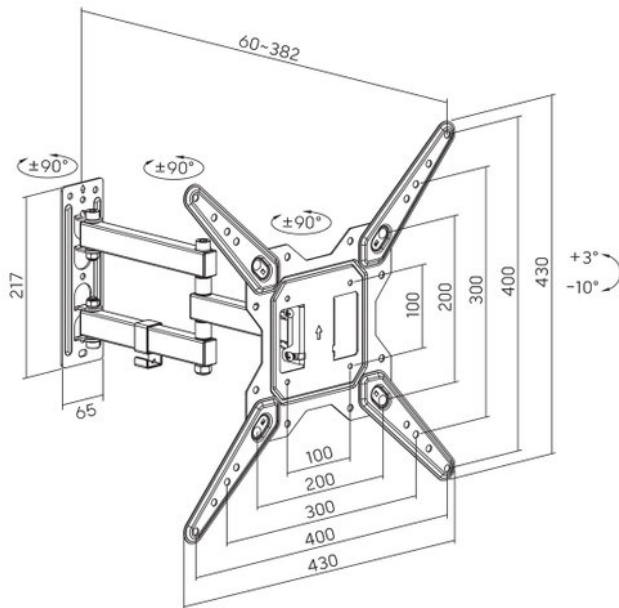
Dimensions (mm)
